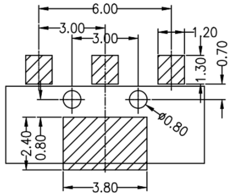
RECOMMENDED PCB LAYOUT TOL:(±0.05)
